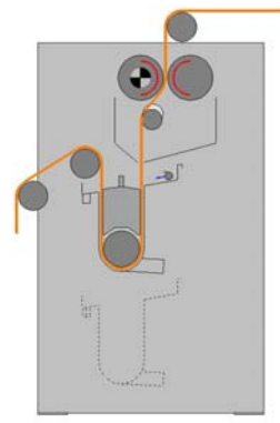
Fabric guiding for nip dyeing
