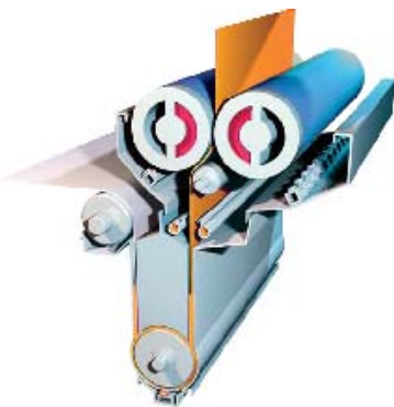
3D cut padder 222.13
