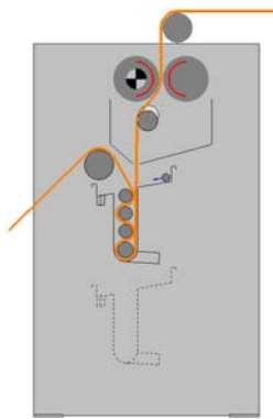
Fabric guiding with underliquor squeezer
